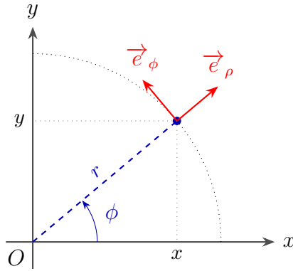
Figura 3.1: Polar coordinates.
